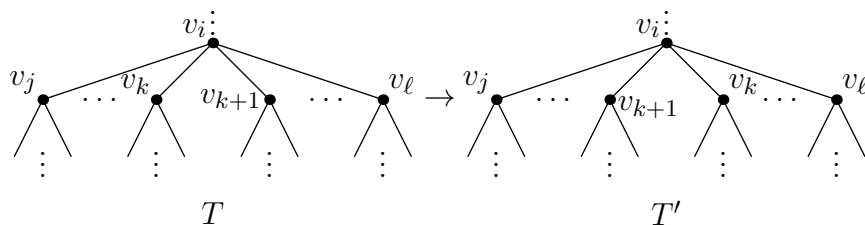
FIGURE 2. Swapping the ordering of two vertices
