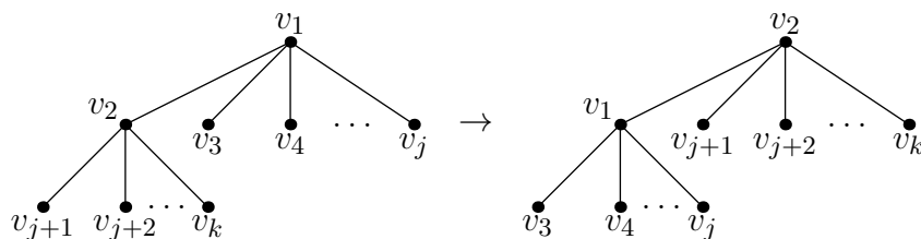
FIGURE 1. Moving the root down an edge
